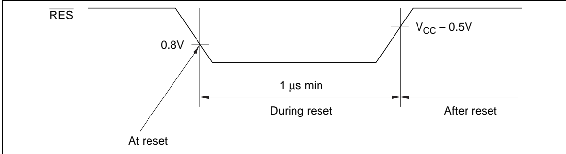
Figure 35 Reset Definition
