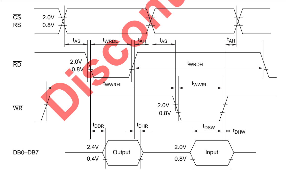
Figure 36 CPU Interface
